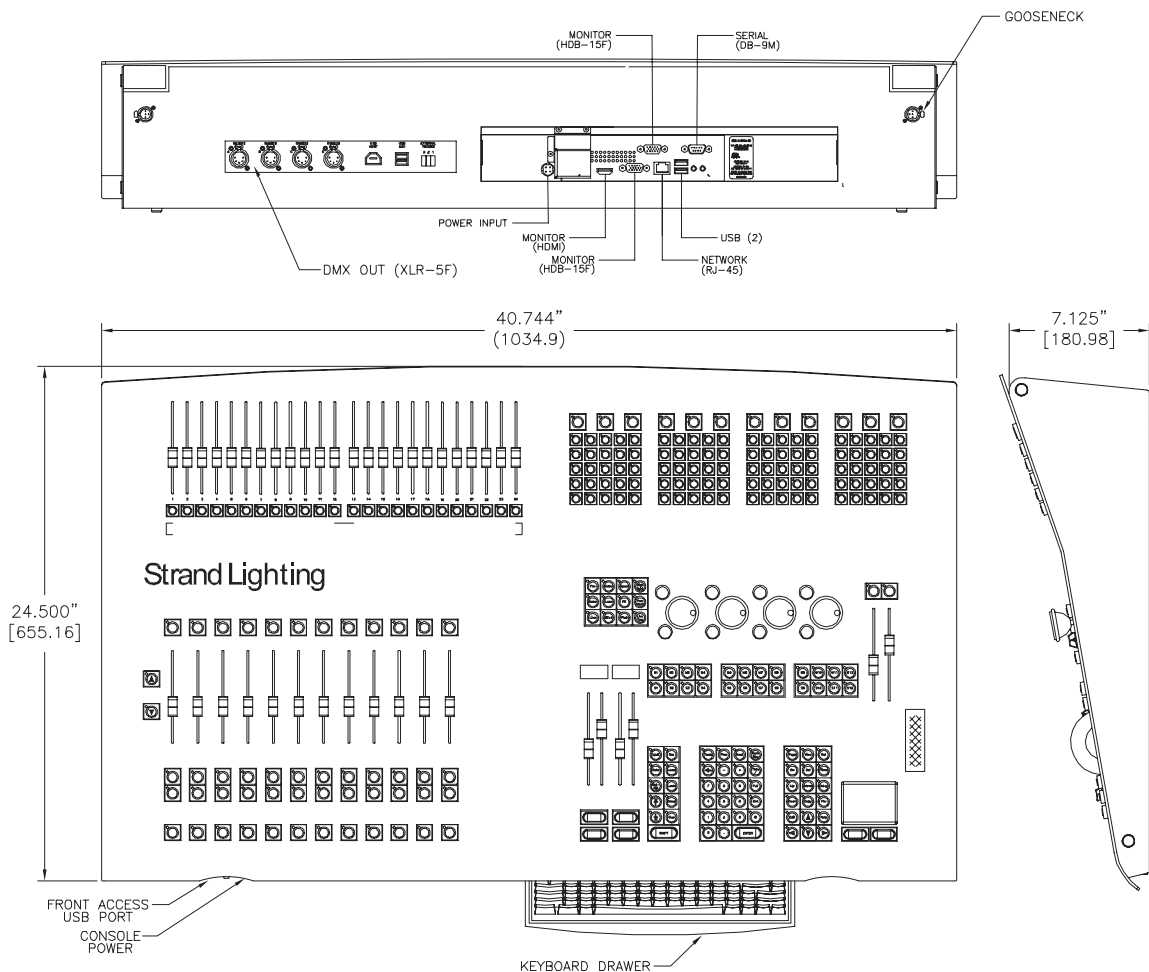
Light Palette VL Lighting Control Console
