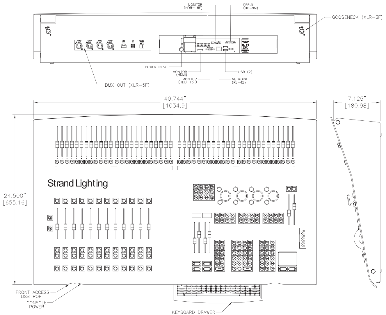
Light Palette Live Lighting Control Console
